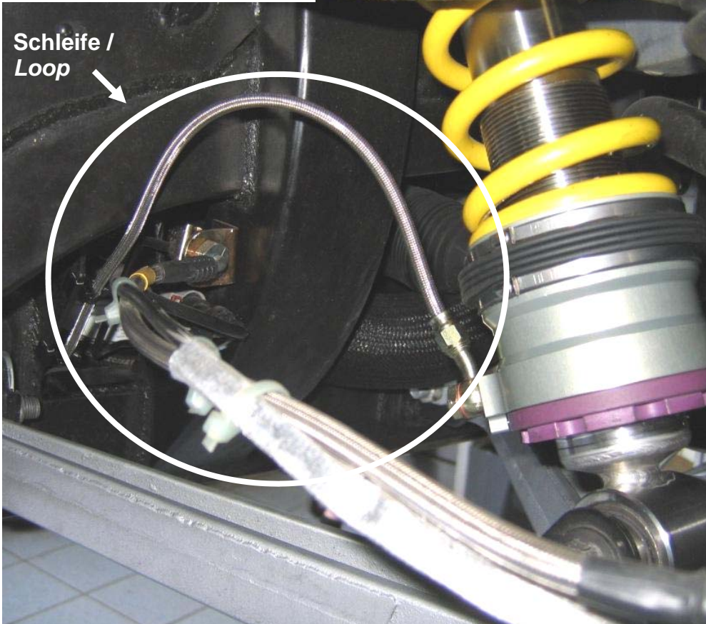
Montageposition 1 / Assembly position 1
