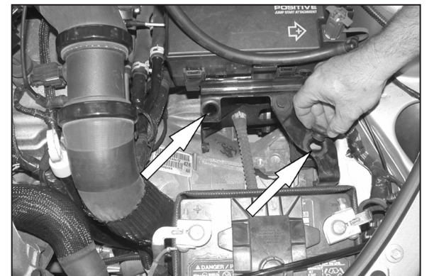
7. Remove the two air box grommets from the stock air box mounting tray.
