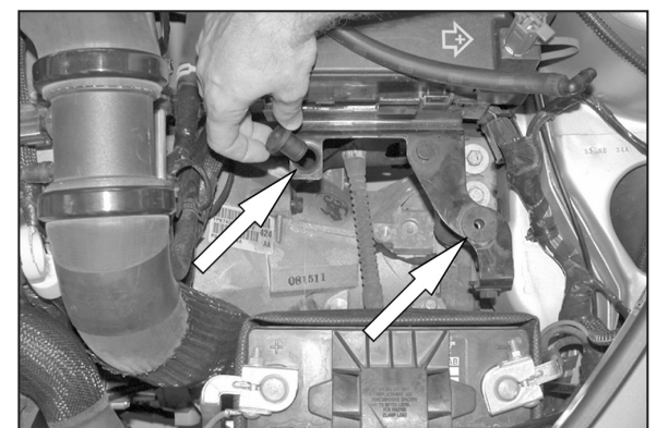
9. Install the two rubber nut inserts into air box grommet holes as shown.
